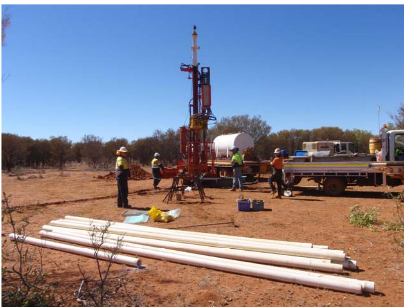
Geotechnical core drilling at the site of the Nolans process plant
